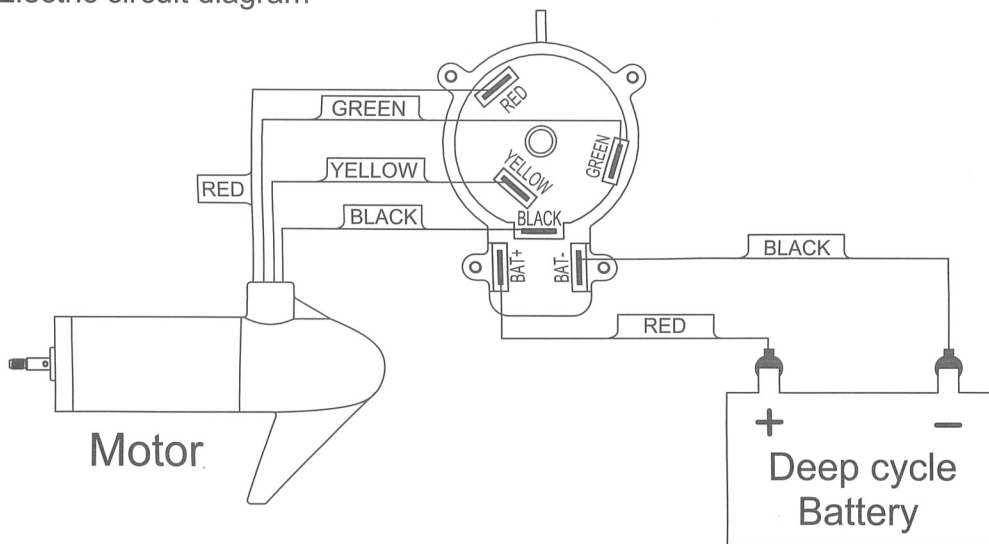
Electric circuit diagram
