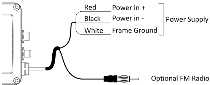
Figure 3 Wiring Instructions
