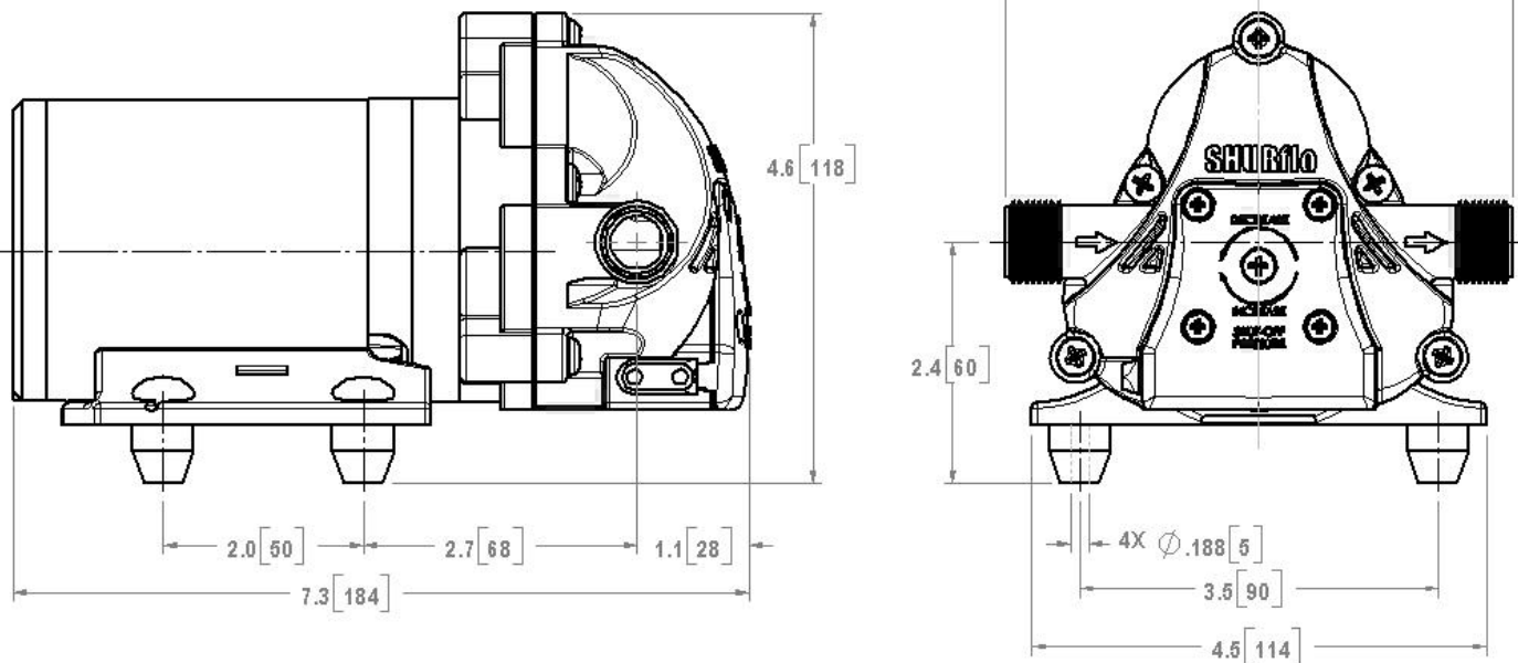
DIMENSIONS [mm]
