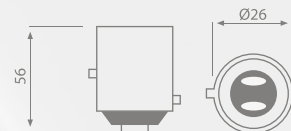
BAY 15d
