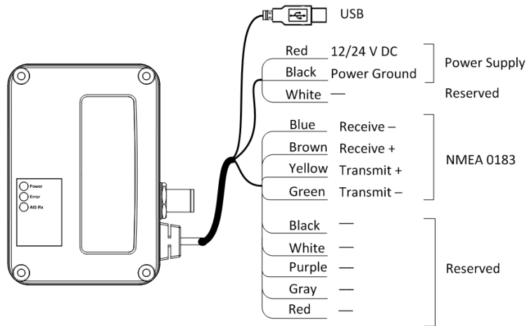
Figure 7 Wiring Instructions
