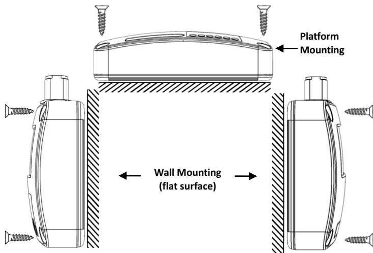
Figure 3 Mounting Instructions (1)
