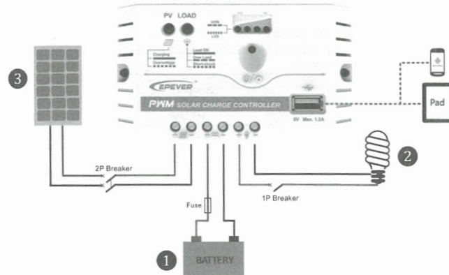
Figure 2 Connection diagram
